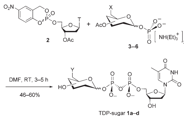
Scheme 3. Synthesis of the NDP sugars starting from the cycloSal phosphate triester.
