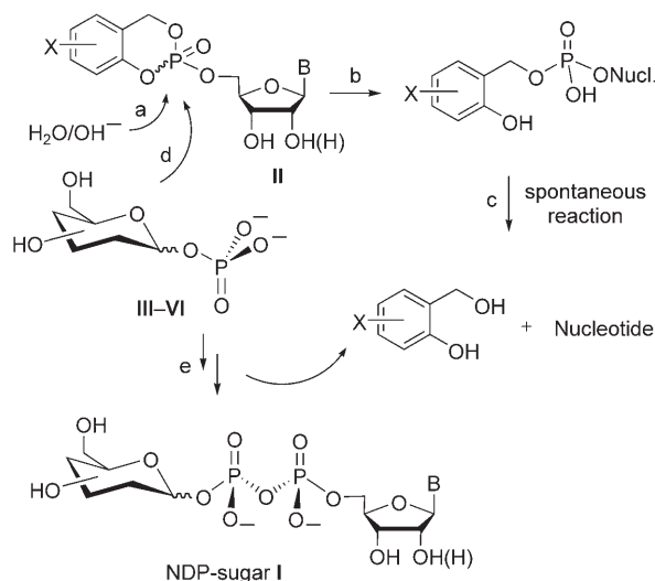
Scheme 1. General principle of the cleavage of cyclo Sal phosphate triesters using water/hydroxide or pyranose 1-phosphates. See text for details.
