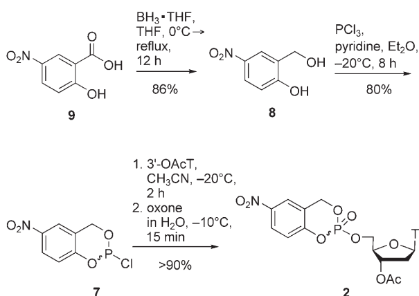
Scheme 2. Synthesis of 5-nitro- cycloSal -(3'-OAc)-thymidine monophosphate.
